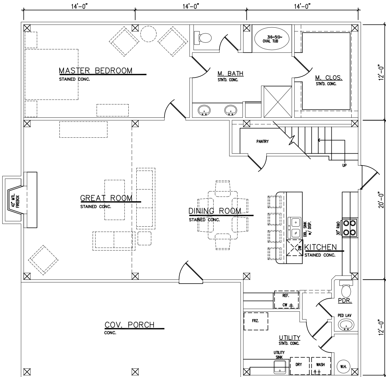
A FIRST FLOOR PLAN Scale: NTS
