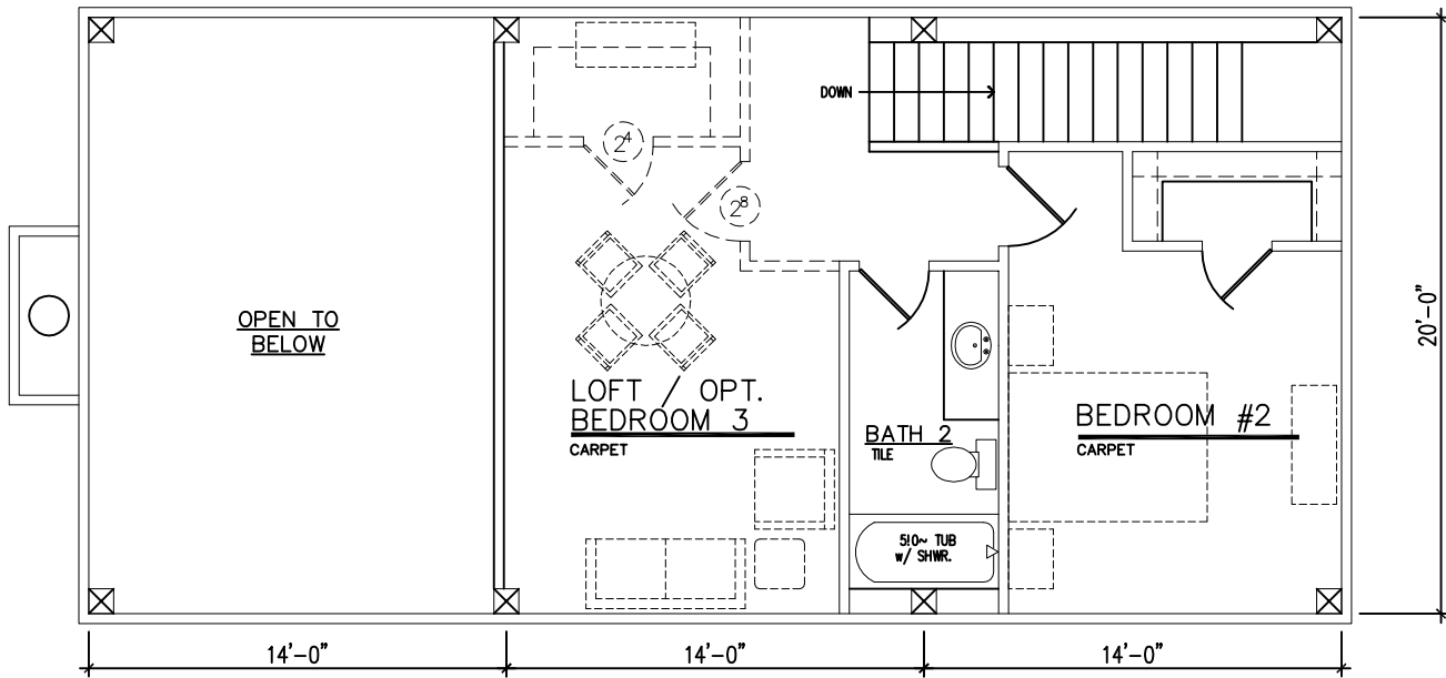
B SECOND FLOOR PLAN Scale: NTS
